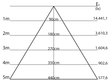
Refleto 60° (ref. 6011-8001) 60° Reflector
